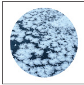
snow emerges on the ice/on top
